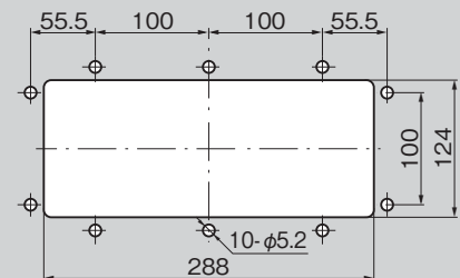
패널 구멍 치수(1/2) Panel drilling dimensions
