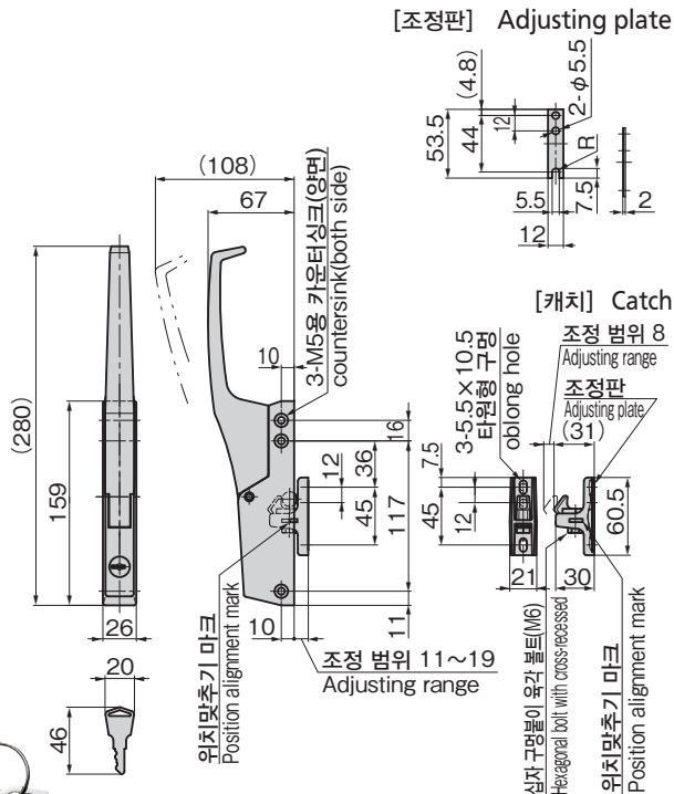
[조정판] Adjusting plate
