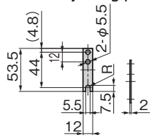
[조정판] Adjusting plate
