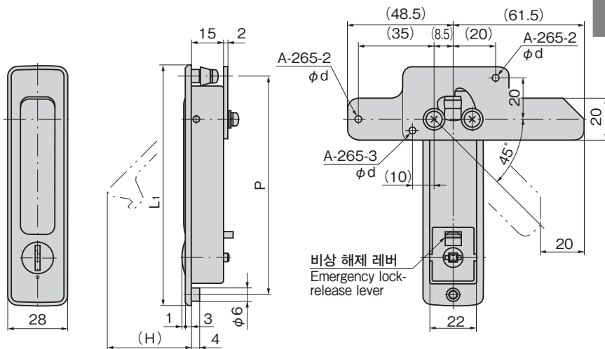
비상해제 레버(뒷면) Emergency lock-release lever (Rear)
