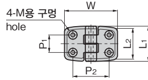
BP-19-1-2-S 접시머리 나사용 For countersink screw
