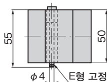
E형 고정링(B-1024-3)용 홈(공칭 3) Groove for E-shaped retaining ring (nominal 3)
