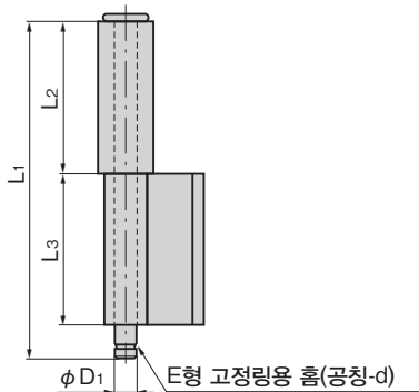
E형 고정링용 홈(공칭-d) Groove for E-shaped retaining ring (nominal-d)
