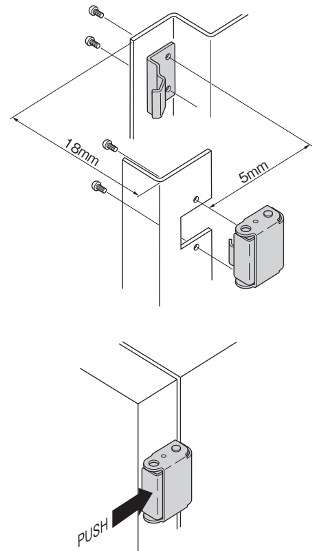
부착 방법 Installation method [C-1017-B]
