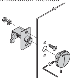
부착 방법 Installation method
