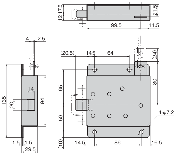
C-1373SD-L
