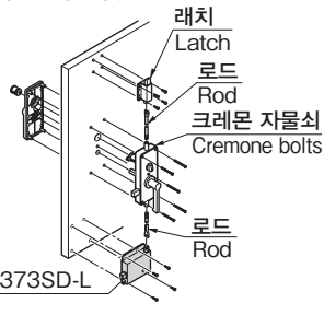
래치 C-1373SD-L Latch
