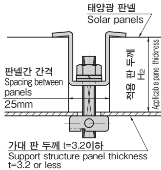
부착 방법(C-1563-H) Installation method
