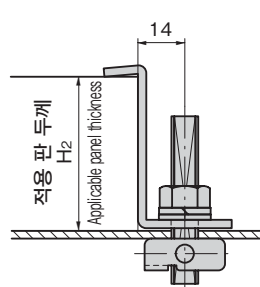
부착 방법(C-1563-Z) Installation method
