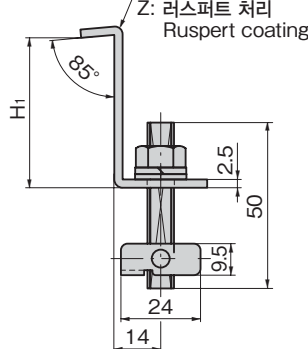
부착 방법(C-1563-Z) Installation method
