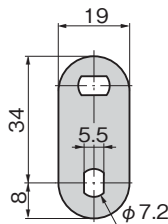
판 두께 t=2.3 Plate thickness
