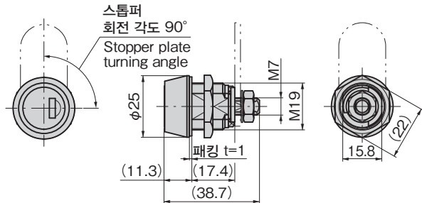
스톱퍼(검용형) Stopper plate (combined-use type)
