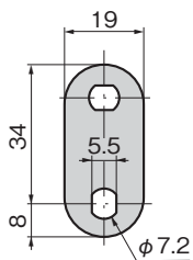
판 두께 t=2.3 Plate thickness
