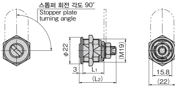
스톱퍼(겸용형) Stopper plate (combined-use type)
